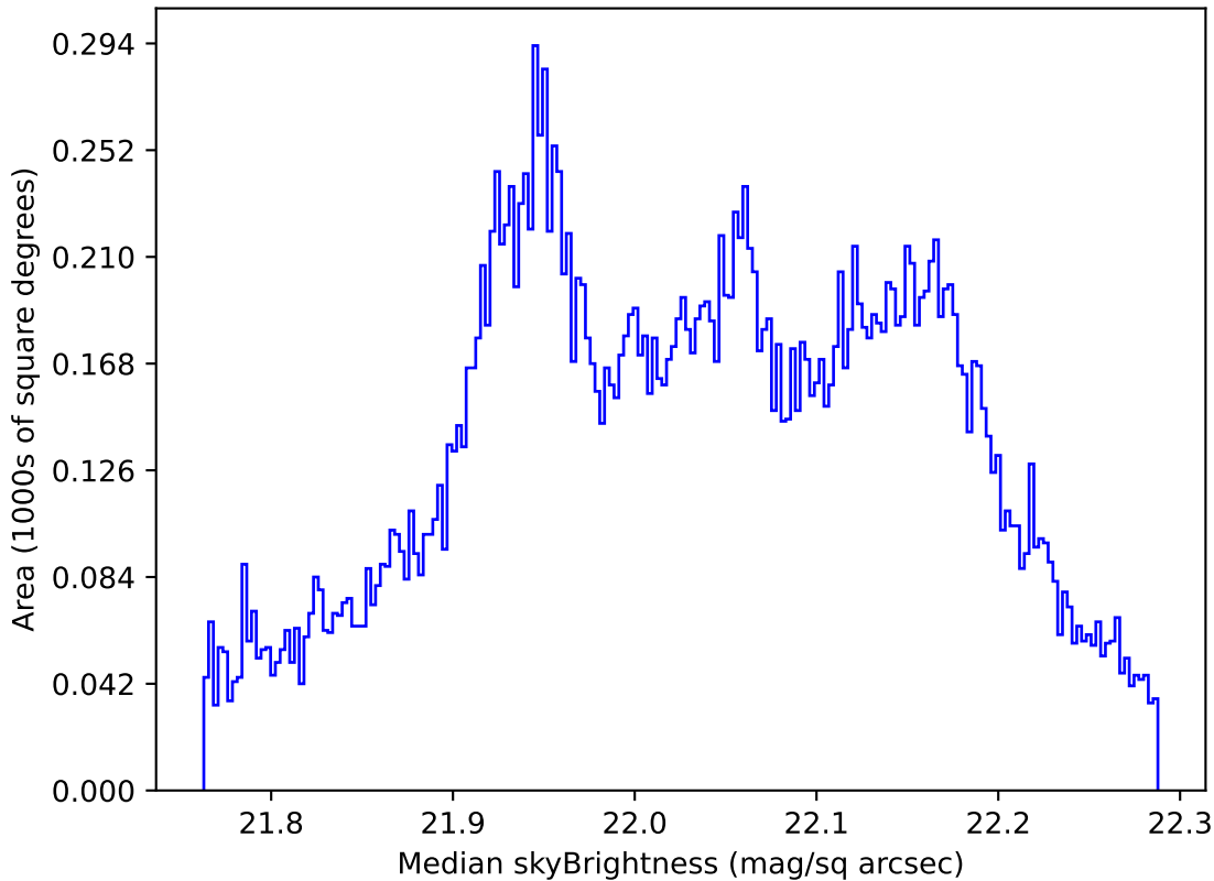
too_elab_r16_d2_griz_v3.4_10yrs All sky g band: Median skyBrightness
