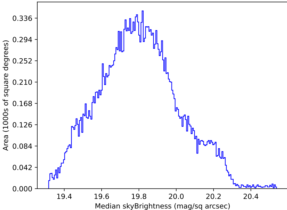
too_elab_r16_d2_griz_v3.4_10yrs All sky all bands: Median skyBrightness
