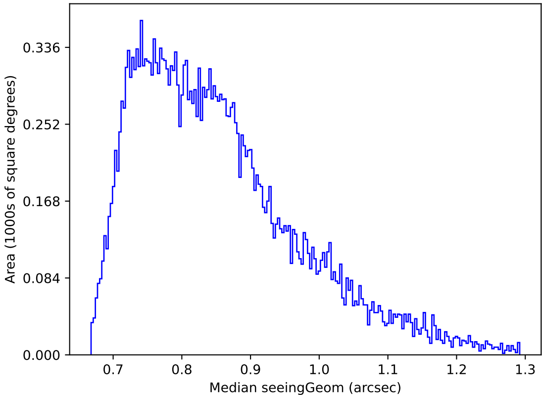
too_elab_r16_d2_griz_v3.4_10yrs Yr 1 r band: Median seeingGeom
