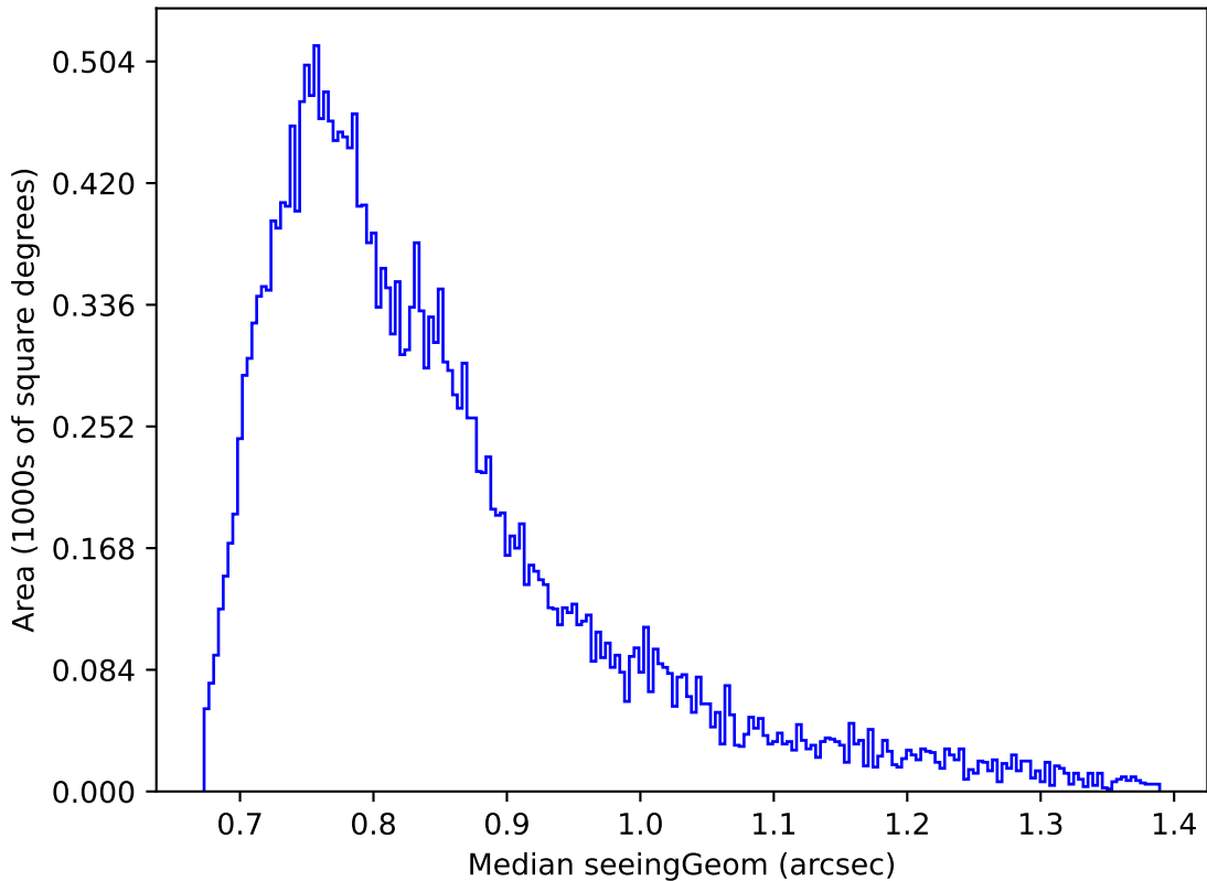
too_elab_r16_d2_griz_v3.4_10yrs Yr 1 i band: Median seeingGeom
