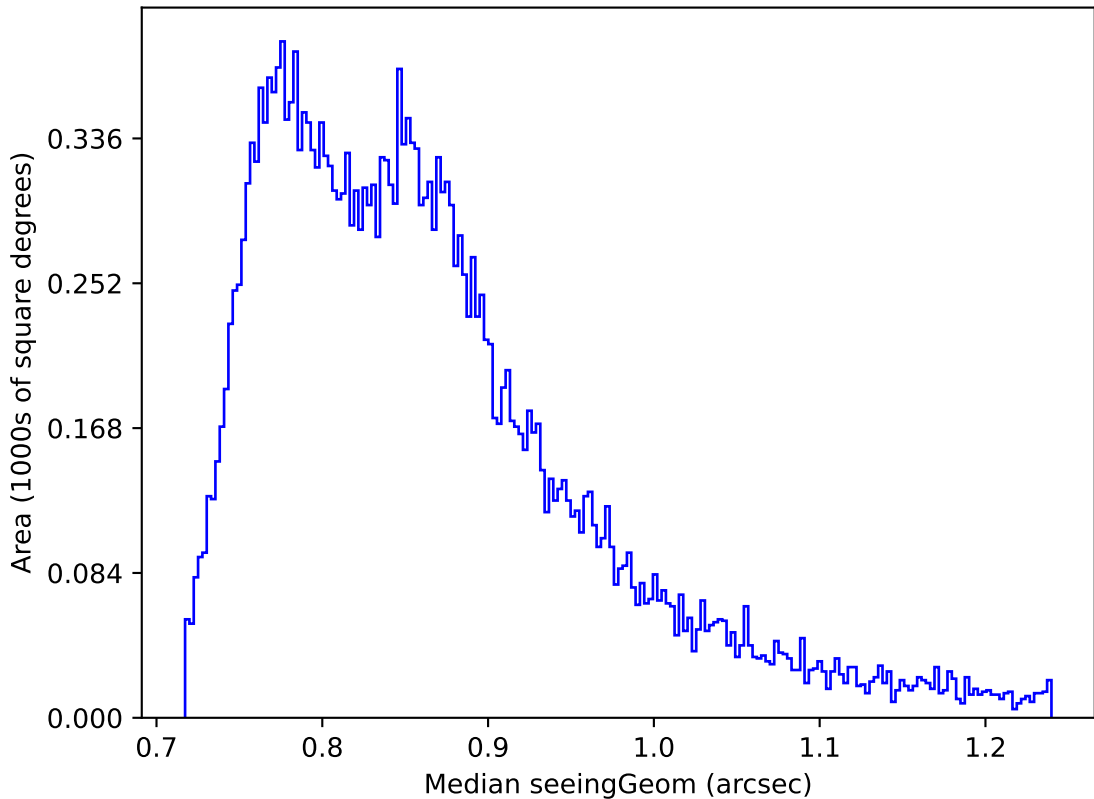
too_elab_r16_d2_griz_v3.4_10yrs Yr 1 all bands: Median seeingGeom
