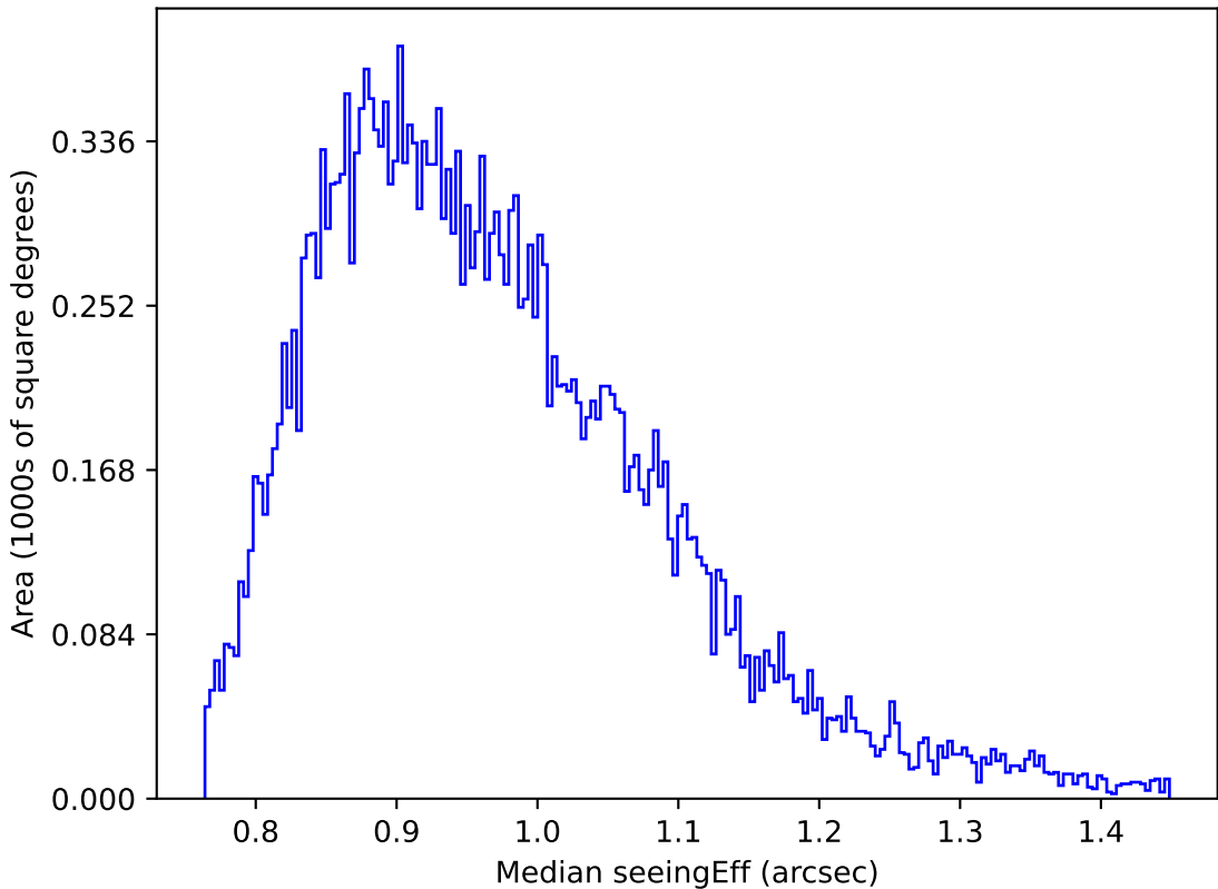
too_elab_r16_d2_griz_v3.4_10yrs Yr 1 z band: Median seeingEff
