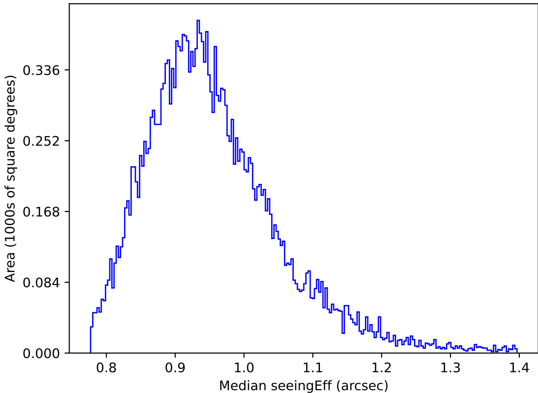
too_elab_r16_d2_griz_v3.4_10yrs Yr 1 y band: Median seeingEff
