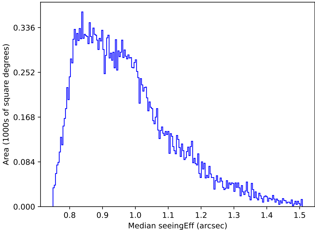
too_elab_r16_d2_griz_v3.4_10yrs Yr 1 r band: Median seeingEff
