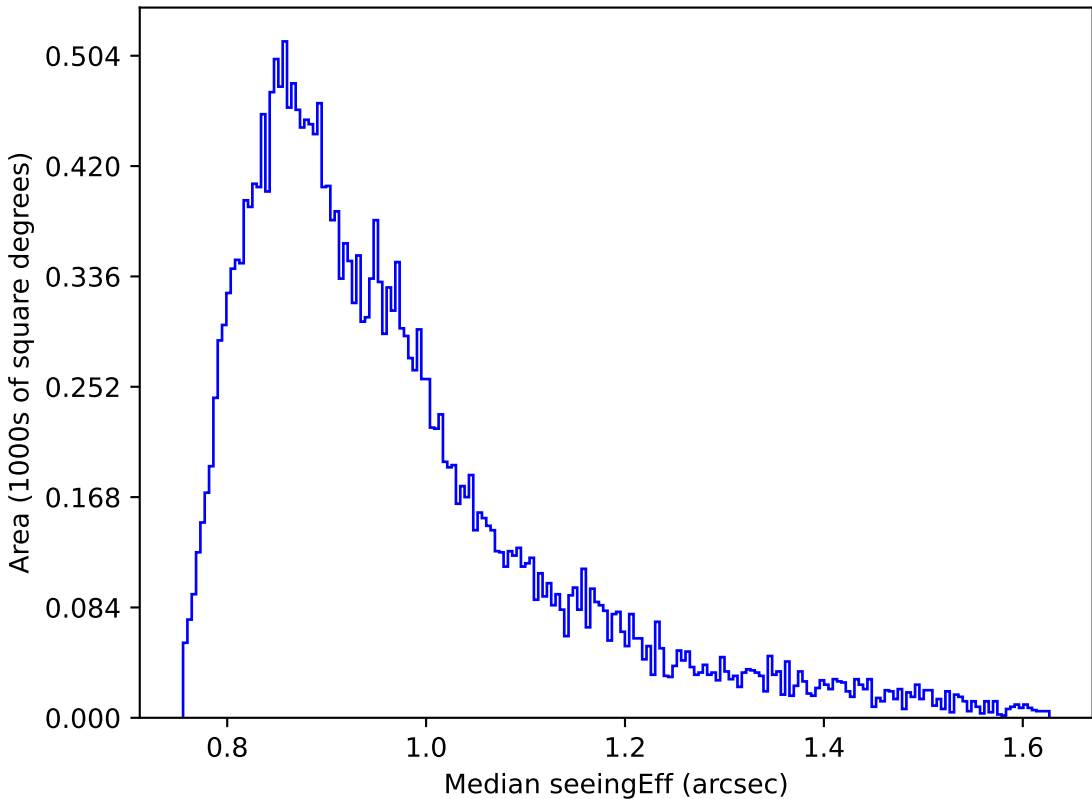
too_elab_r16_d2_griz_v3.4_10yrs Yr 1 i band: Median seeingEff
