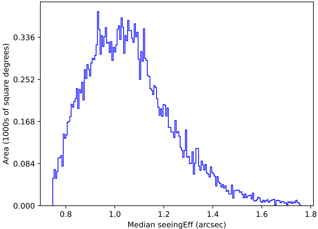
too_elab_r16_d2_griz_v3.4_10yrs Yr 1 g band: Median seeingEff
