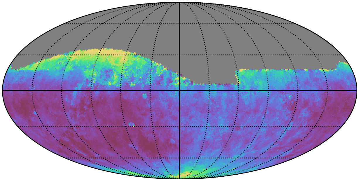
too_elab_r16_d2_griz_v3.4_10yrs Yr 1 all bands: Median seeingEff
