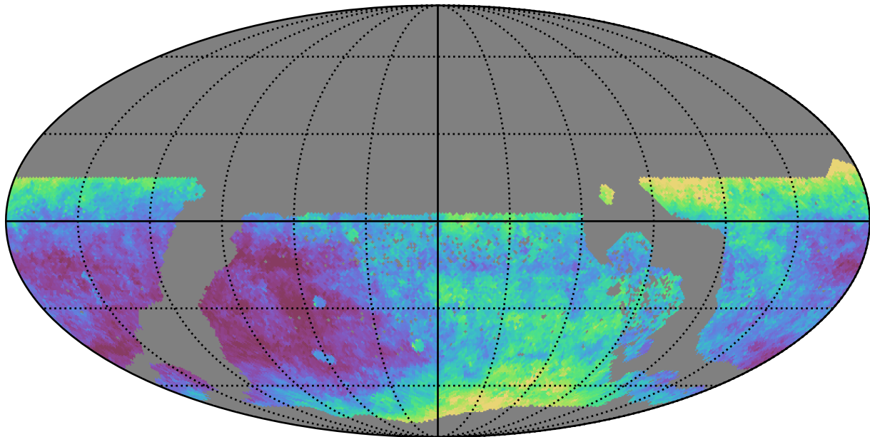
too_elab_r16_d2_griz_v3.4_10yrs WFD z band: Median seeingEff
