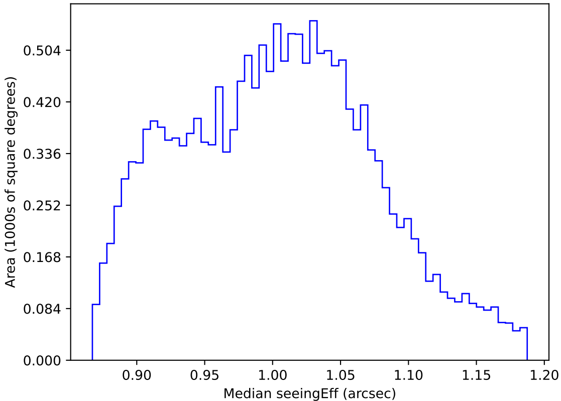
too_elab_r16_d2_griz_v3.4_10yrs WFD z band: Median seeingEff
