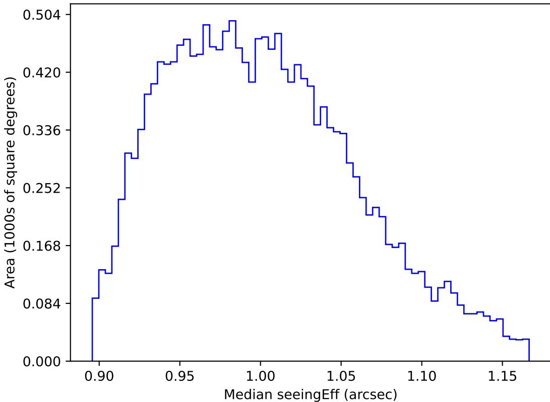
too_elab_r16_d2_griz_v3.4_10yrs WFD y band: Median seeingEff
