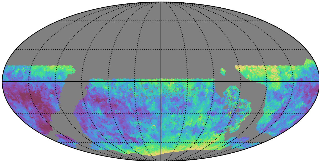
too_elab_r16_d2_griz_v3.4_10yrs WFD u band: Median seeingEff
