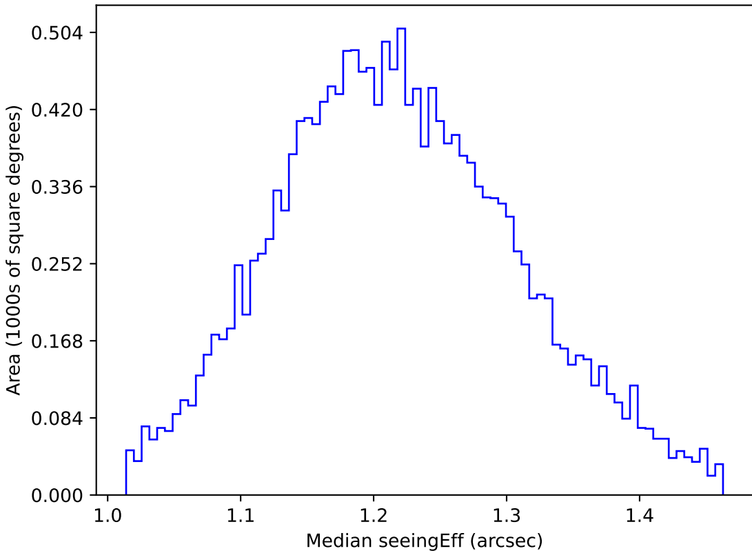
too_elab_r16_d2_griz_v3.4_10yrs WFD u band: Median seeingEff
