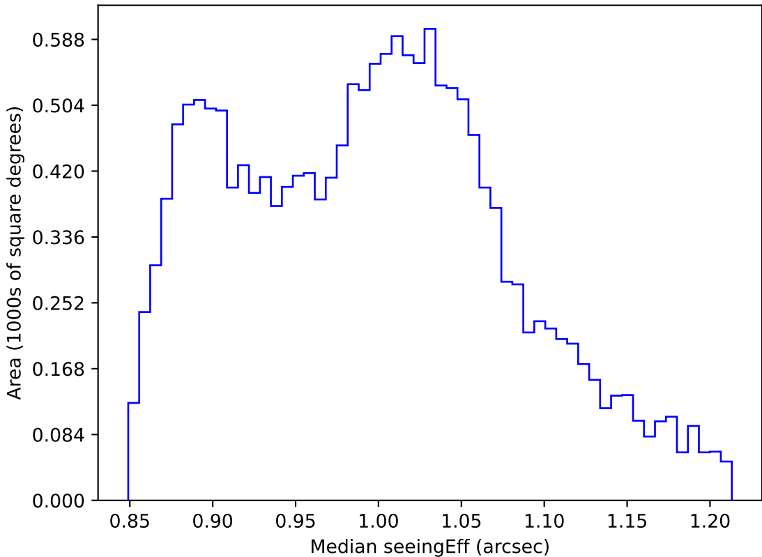
too_elab_r16_d2_griz_v3.4_10yrs WFD i band: Median seeingEff
