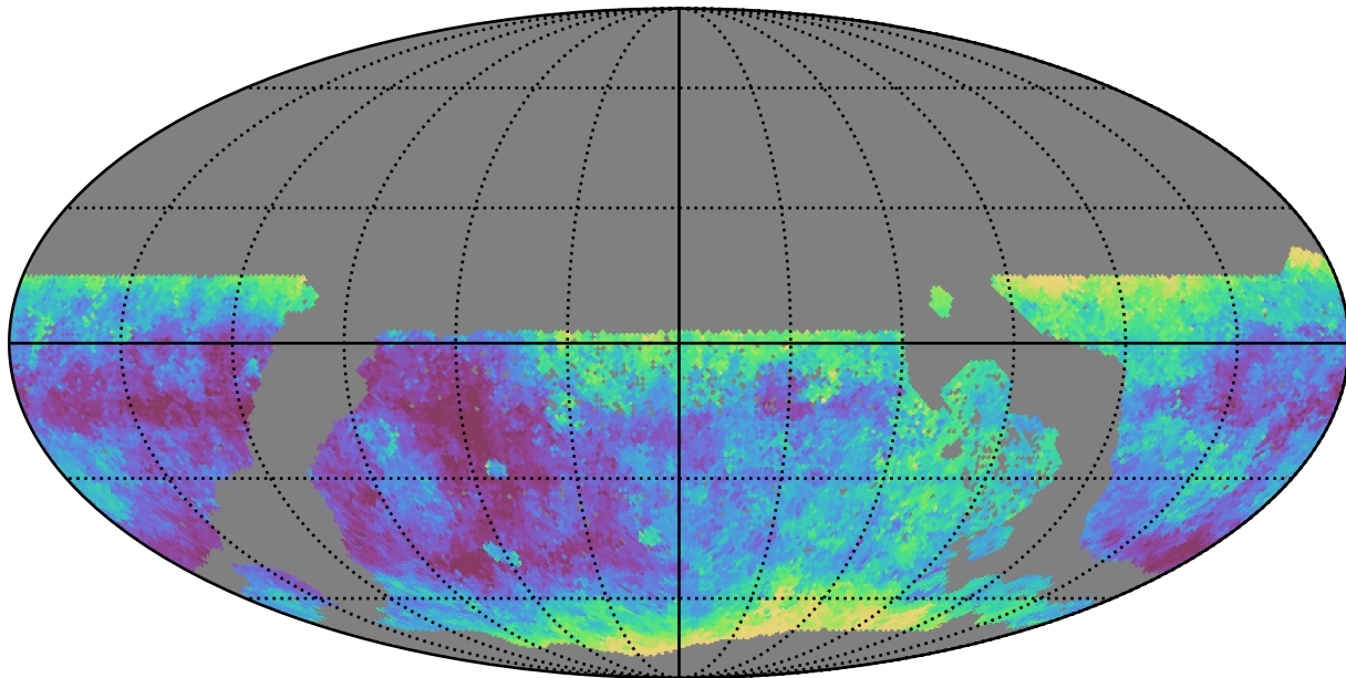
too_elab_r16_d2_griz_v3.4_10yrs WFD g band: Median seeingEff
