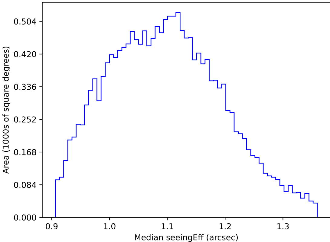
too_elab_r16_d2_griz_v3.4_10yrs WFD g band: Median seeingEff
