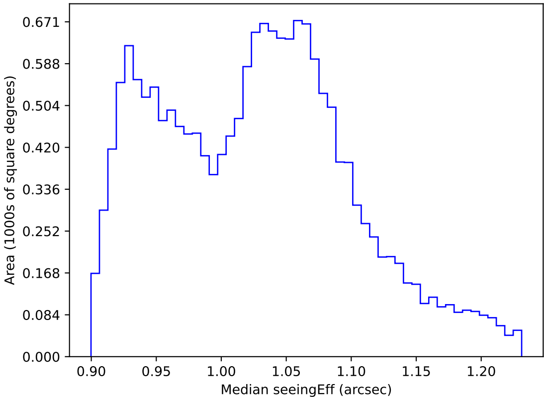
too_elab_r16_d2_griz_v3.4_10yrs WFD all bands: Median seeingEff
