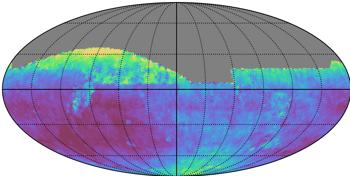
too_elab_r16_d2_griz_v3.4_10yrs All sky z band: Median seeingEff
