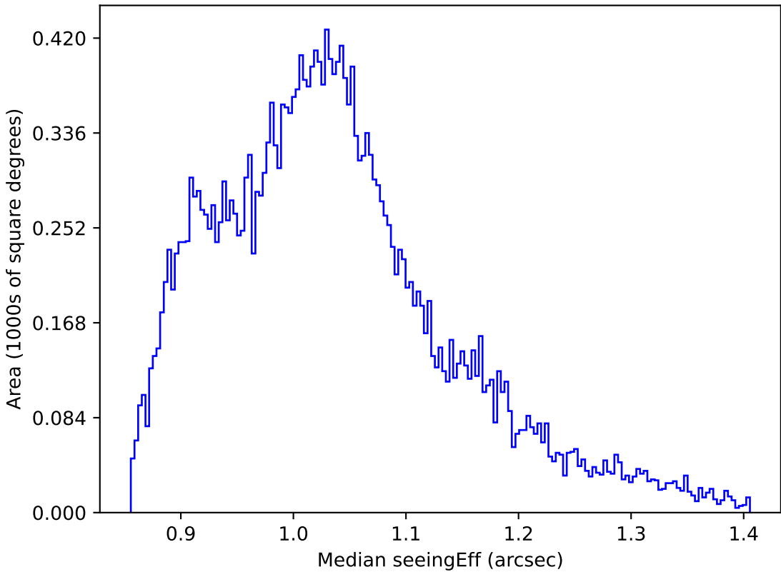
too_elab_r16_d2_griz_v3.4_10yrs All sky z band: Median seeingEff
