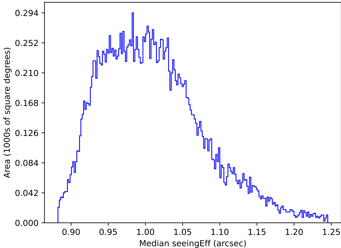
too_elab_r16_d2_griz_v3.4_10yrs All sky y band: Median seeingEff
