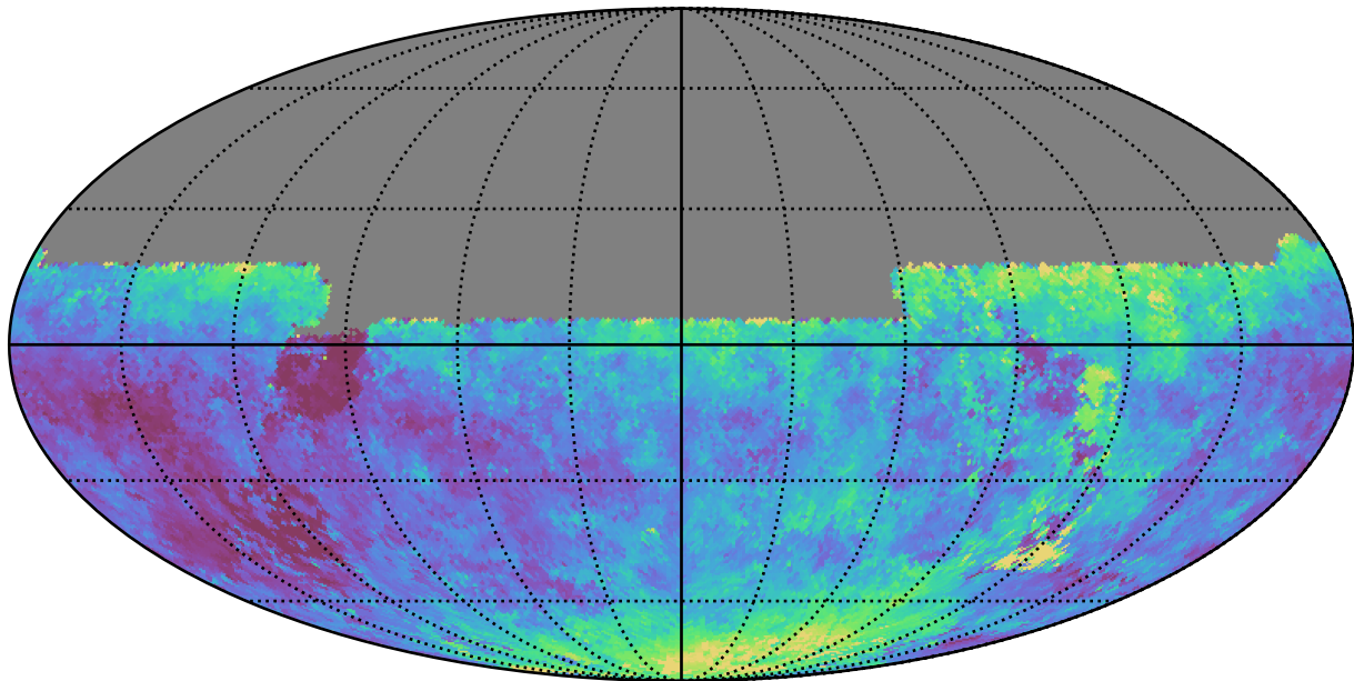
too_elab_r16_d2_griz_v3.4_10yrs All sky u band: Median seeingEff
