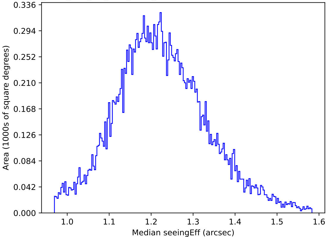
too_elab_r16_d2_griz_v3.4_10yrs All sky u band: Median seeingEff
