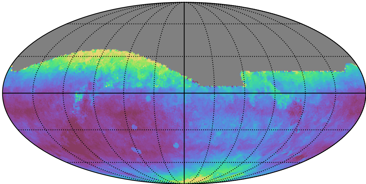
too_elab_r16_d2_griz_v3.4_10yrs All sky r band: Median seeingEff
