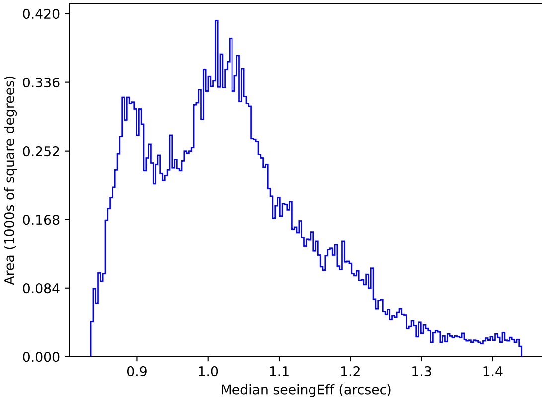
too_elab_r16_d2_griz_v3.4_10yrs All sky i band: Median seeingEff
