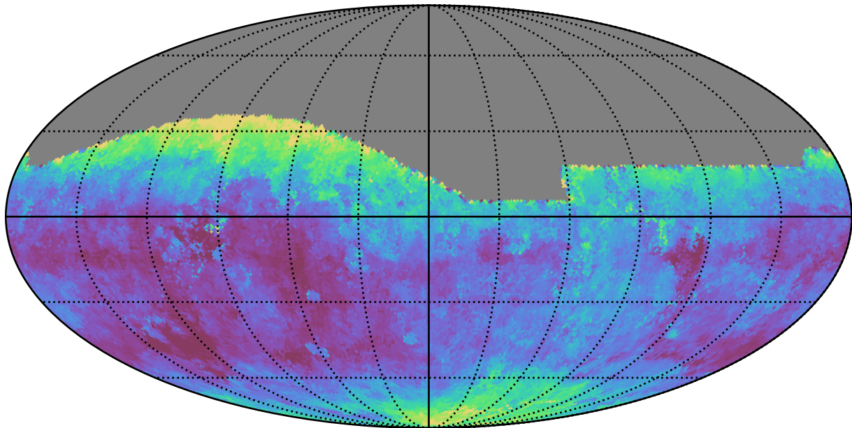
too_elab_r16_d2_griz_v3.4_10yrs All sky g band: Median seeingEff
