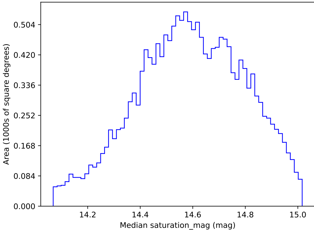
too_elab_r16_d2_griz_v3.4_10yrs WFD g band: Median saturation_mag
