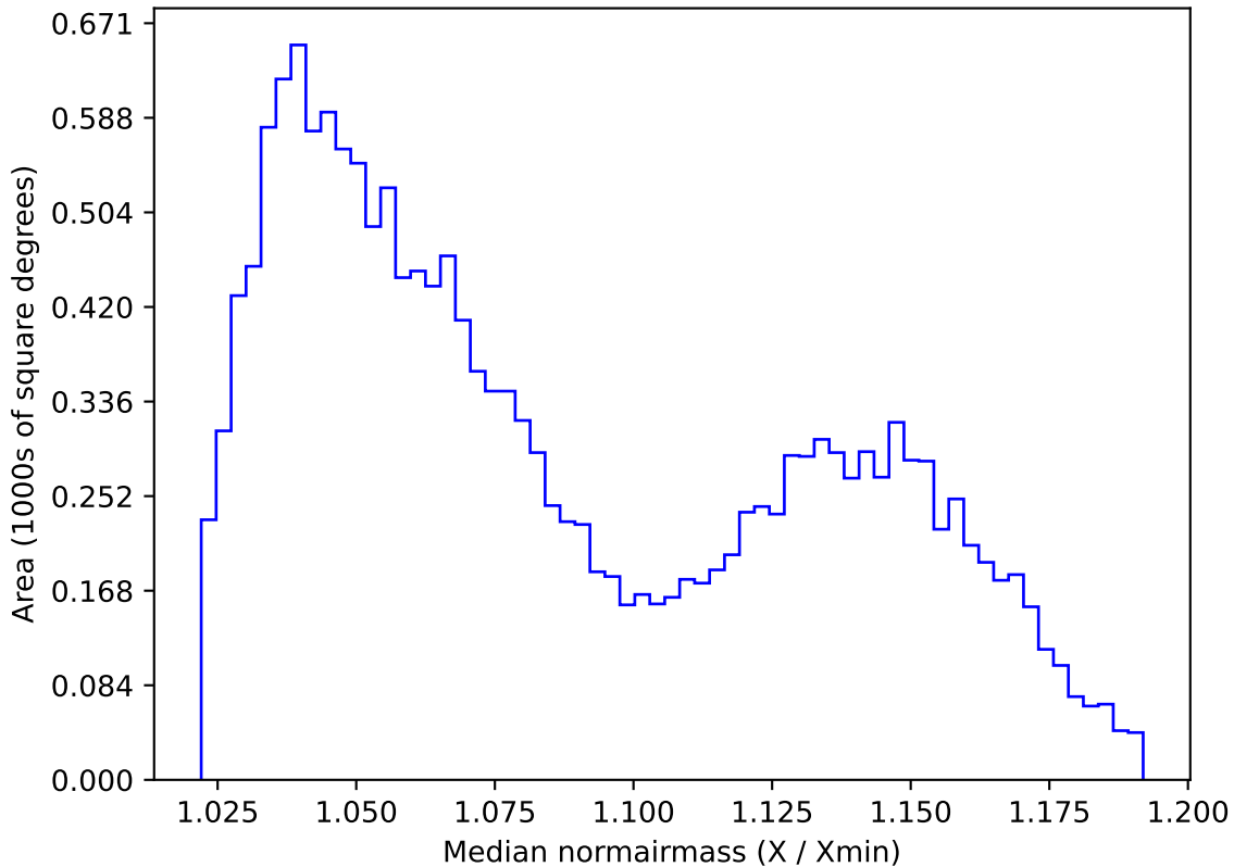
too_elab_r16_d2_griz_v3.4_10yrs WFD z band: Median normairmass
