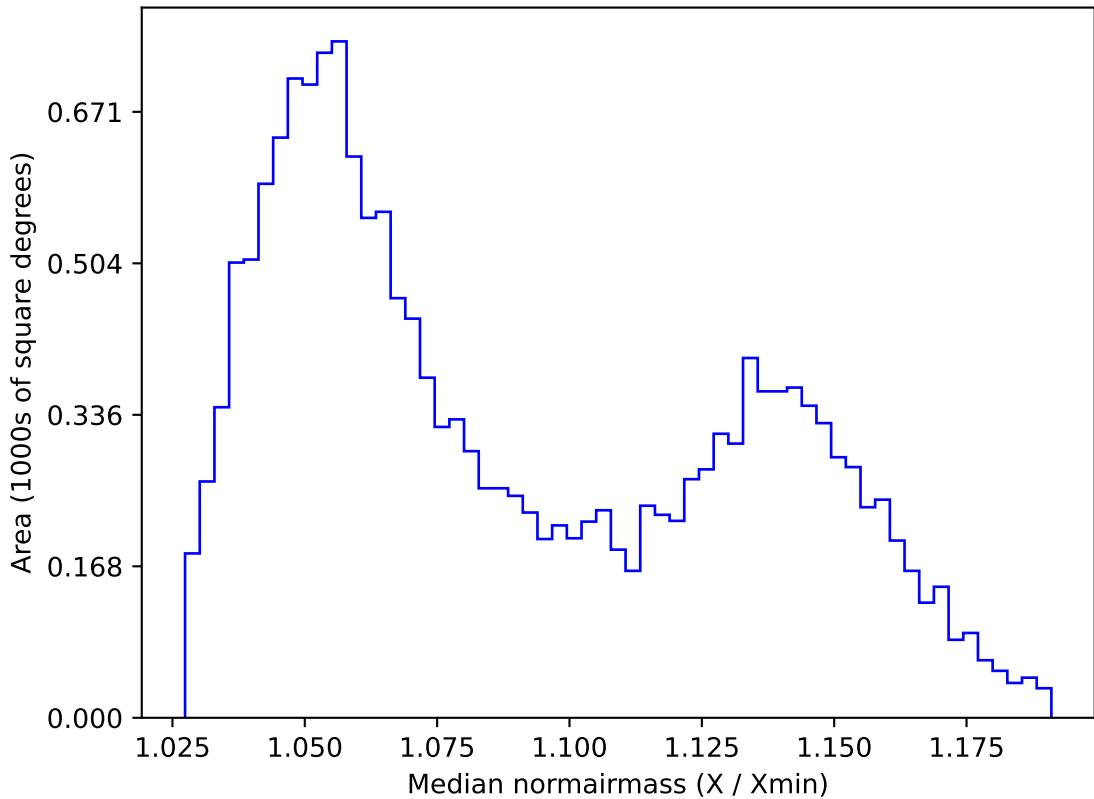
too_elab_r16_d2_griz_v3.4_10yrs WFD y band: Median normairmass
