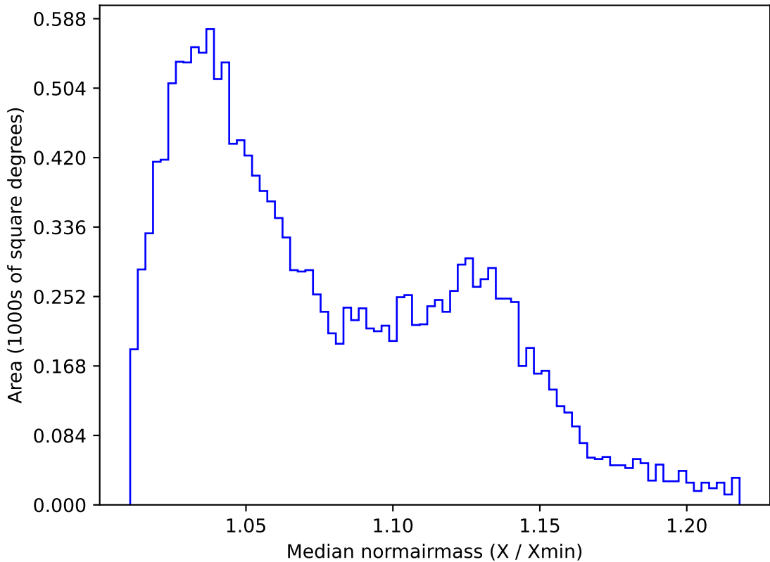
too_elab_r16_d2_griz_v3.4_10yrs WFD u band: Median normairmass
