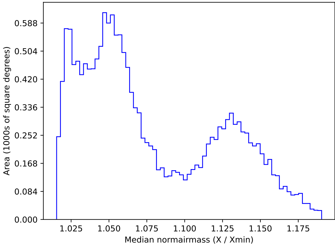
too_elab_r16_d2_griz_v3.4_10yrs WFD r band: Median normairmass
