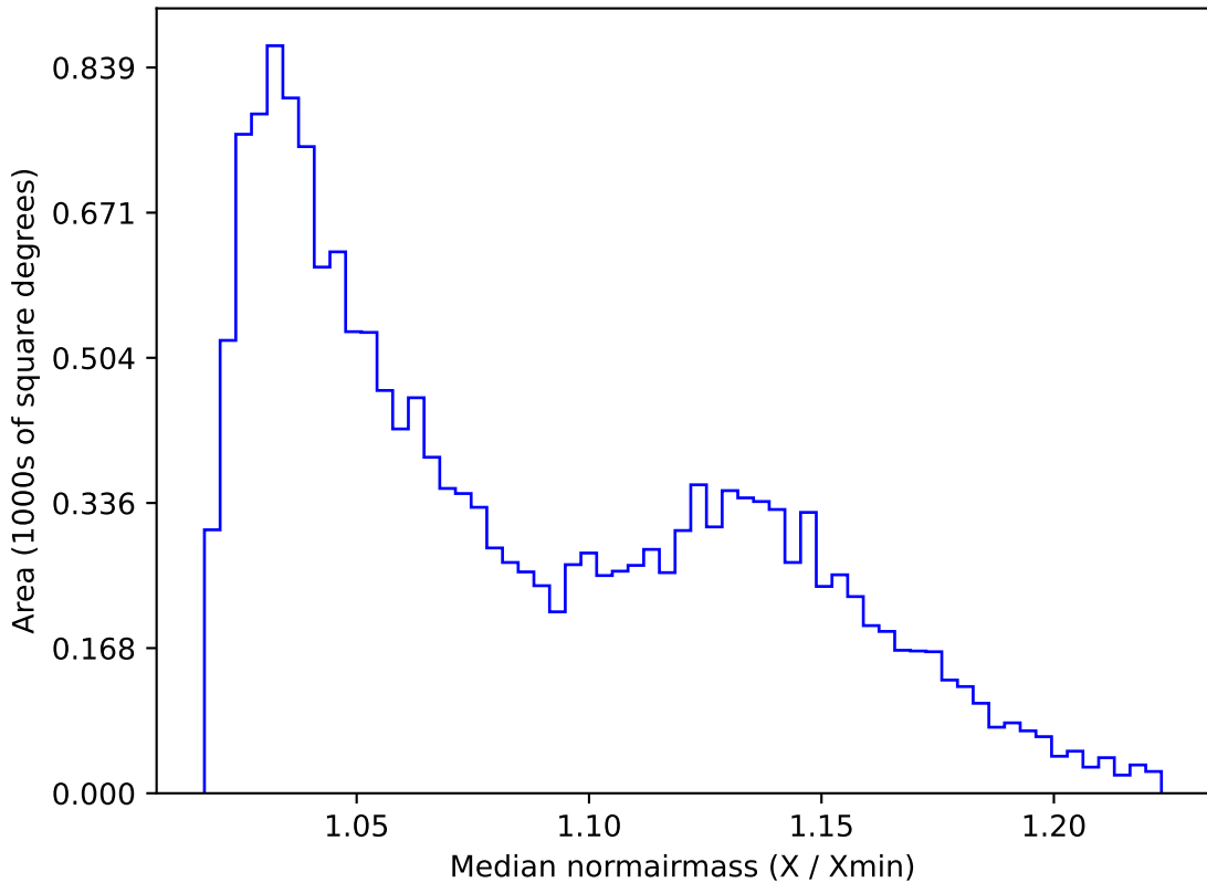
too_elab_r16_d2_griz_v3.4_10yrs WFD g band: Median normairmass
