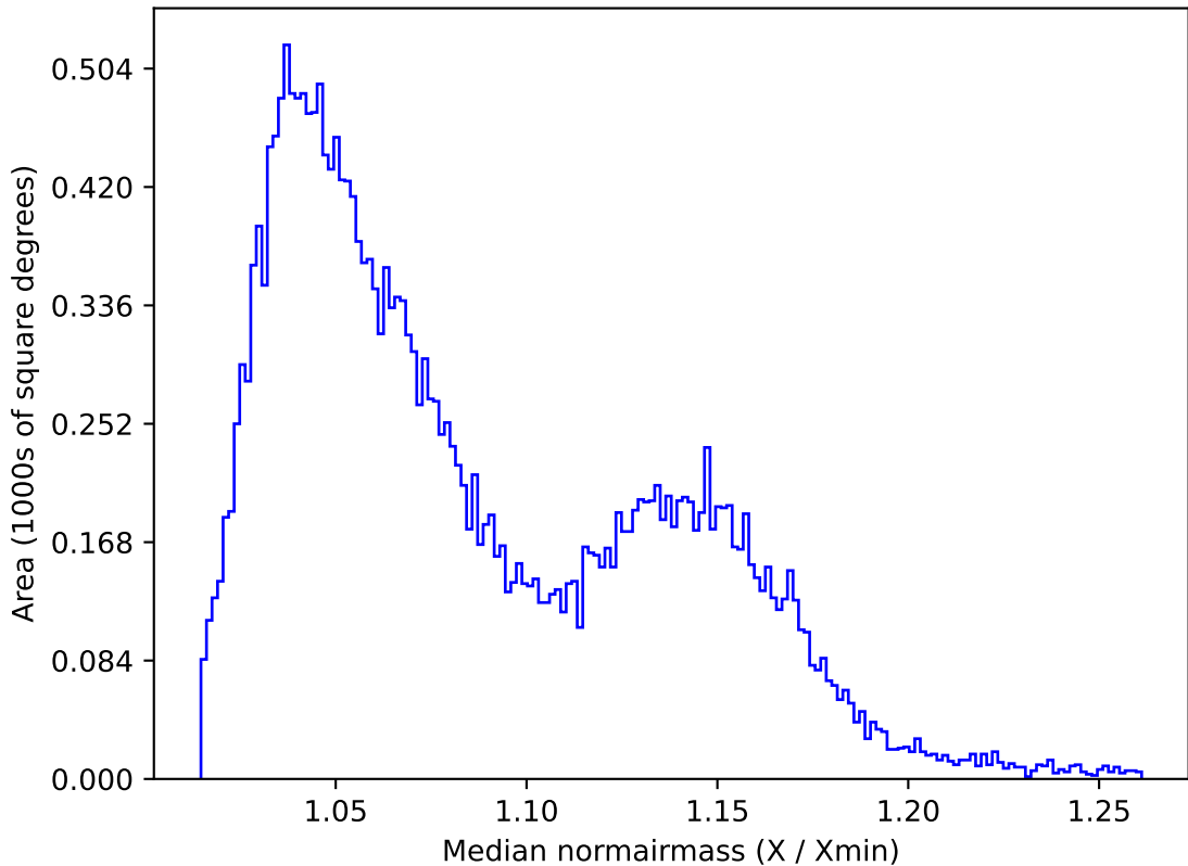
too_elab_r16_d2_griz_v3.4_10yrs All sky z band: Median normairmass
