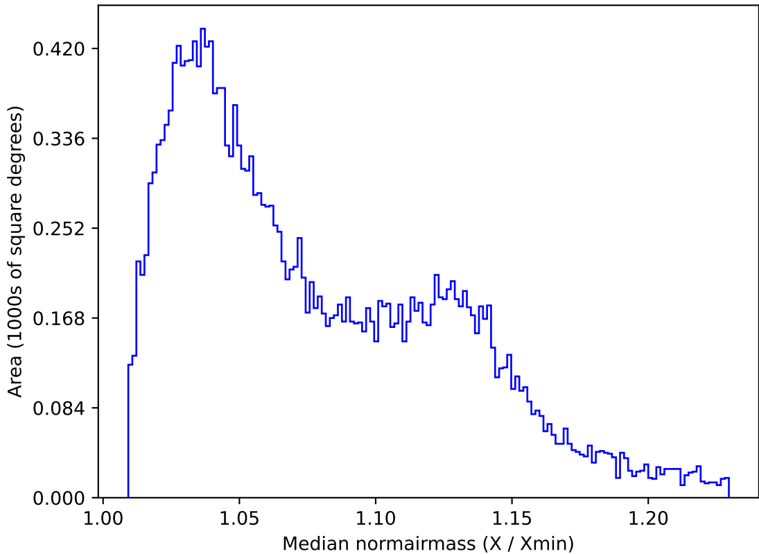
too_elab_r16_d2_griz_v3.4_10yrs All sky u band: Median normairmass
