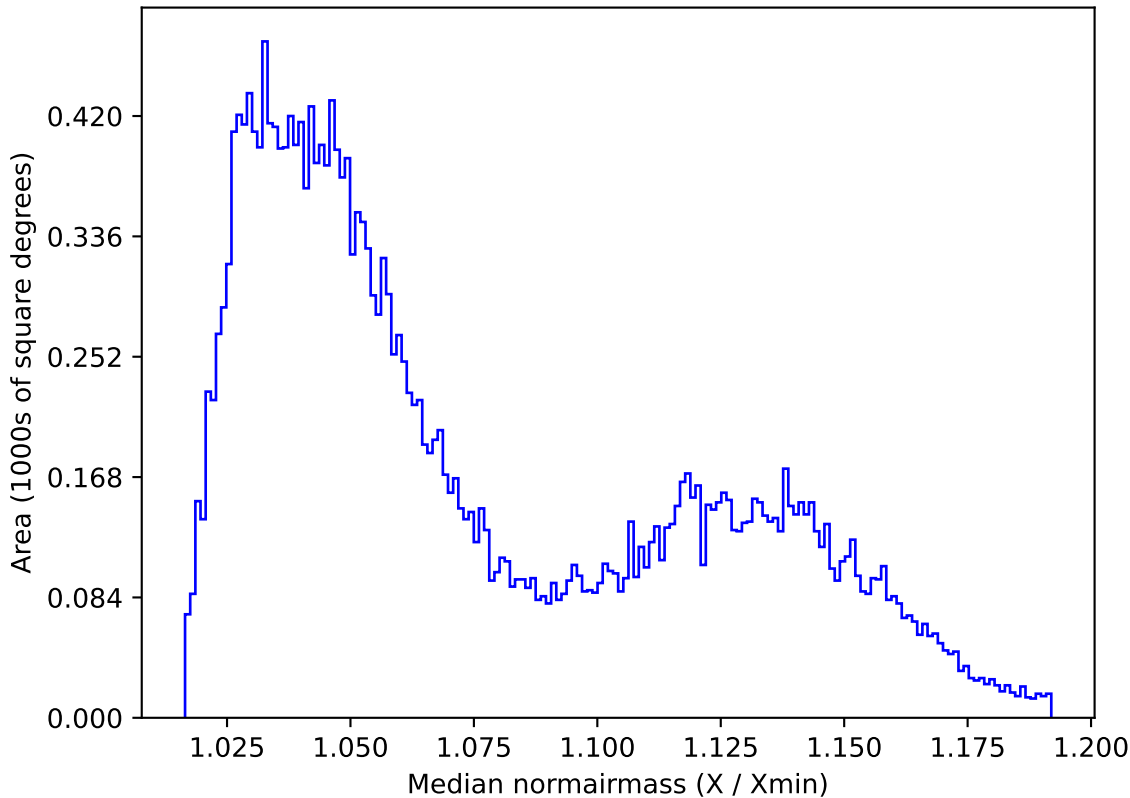
too_elab_r16_d2_griz_v3.4_10yrs All sky i band: Median normairmass
