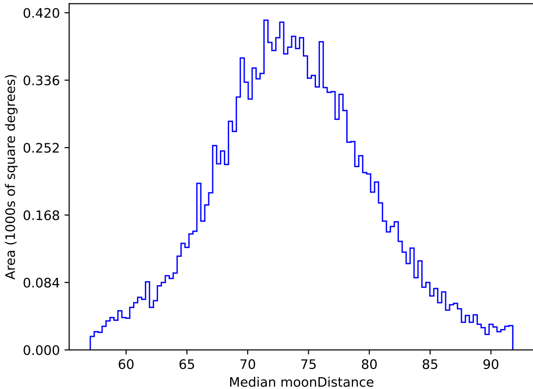
too_elab_r16_d2_griz_v3.4_10yrs WFD z band: Median moonDistance
