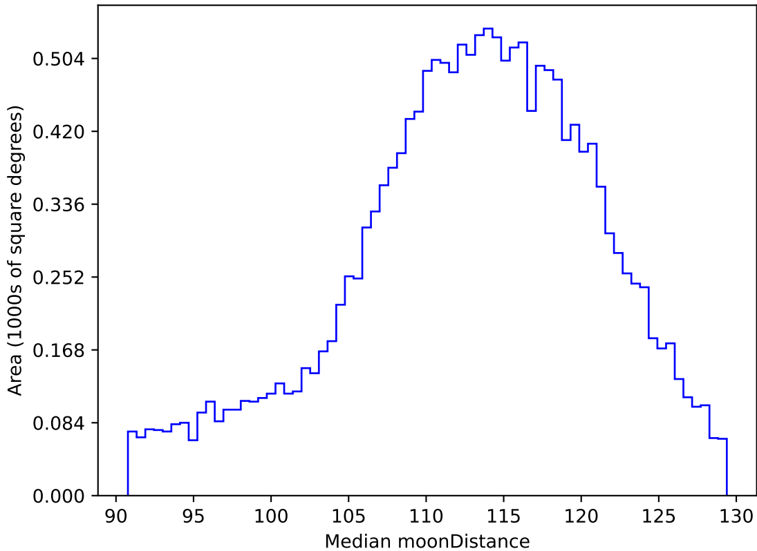
too_elab_r16_d2_griz_v3.4_10yrs WFD r band: Median moonDistance
