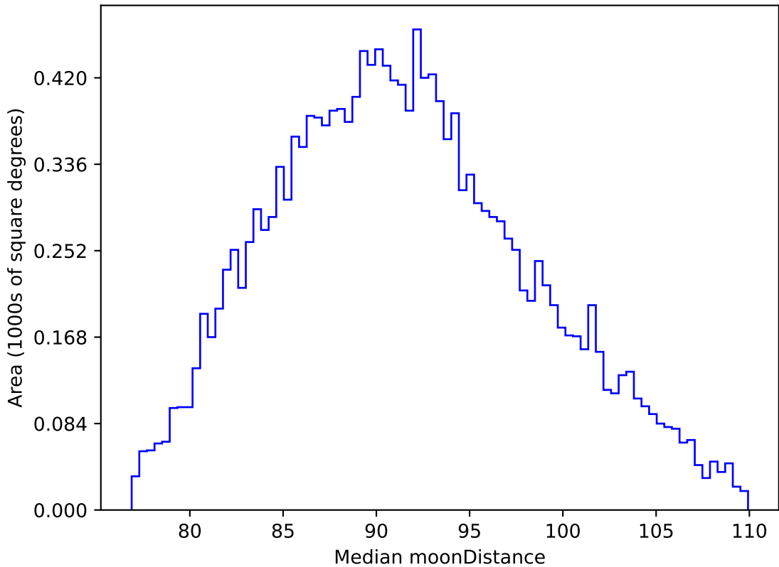
too_elab_r16_d2_griz_v3.4_10yrs WFD i band: Median moonDistance
