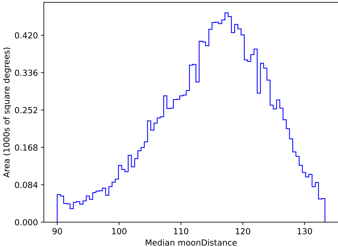
too_elab_r16_d2_griz_v3.4_10yrs WFD g band: Median moonDistance
