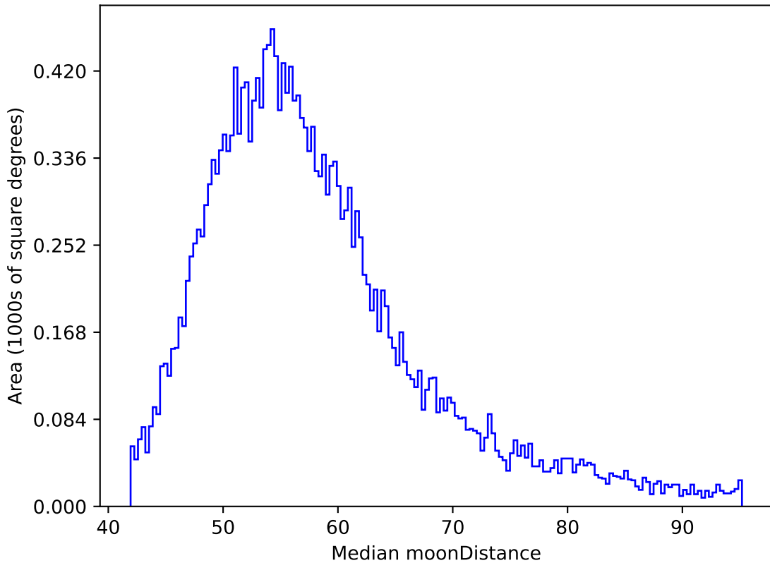
too_elab_r16_d2_griz_v3.4_10yrs All sky y band: Median moonDistance
