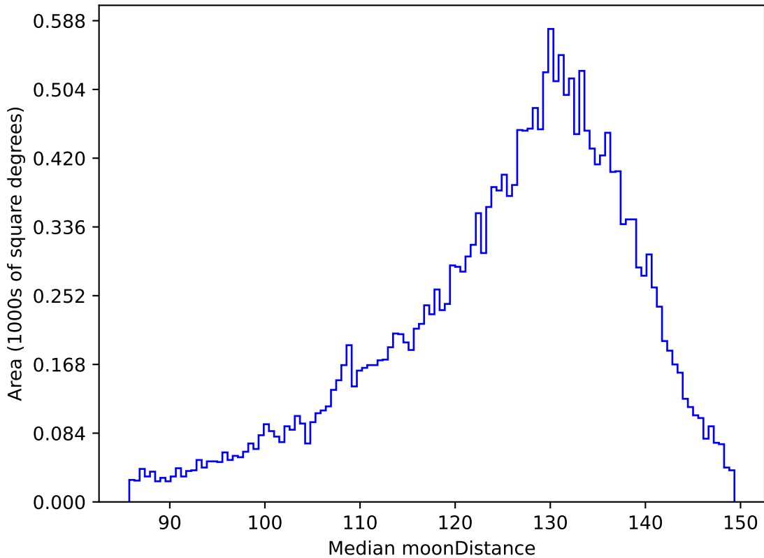
too_elab_r16_d2_griz_v3.4_10yrs All sky u band: Median moonDistance
