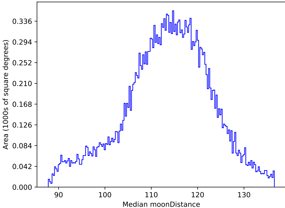
too_elab_r16_d2_griz_v3.4_10yrs All sky r band: Median moonDistance
