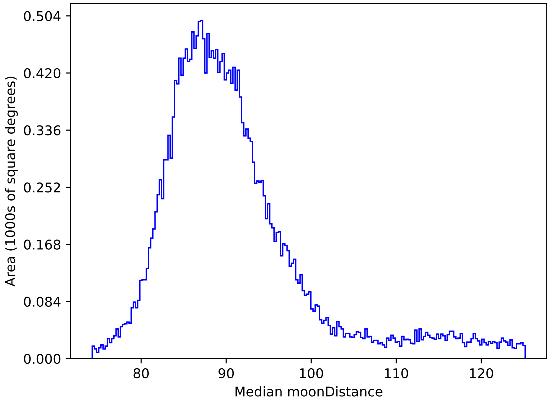
too_elab_r16_d2_griz_v3.4_10yrs All sky all bands: Median moonDistance
