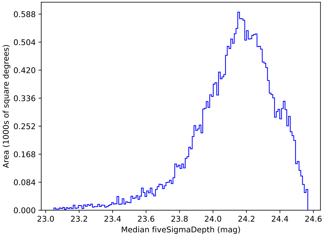
too_elab_r16_d2_griz_v3.4_10yrs Yr 1 r band: Median fiveSigmaDepth
