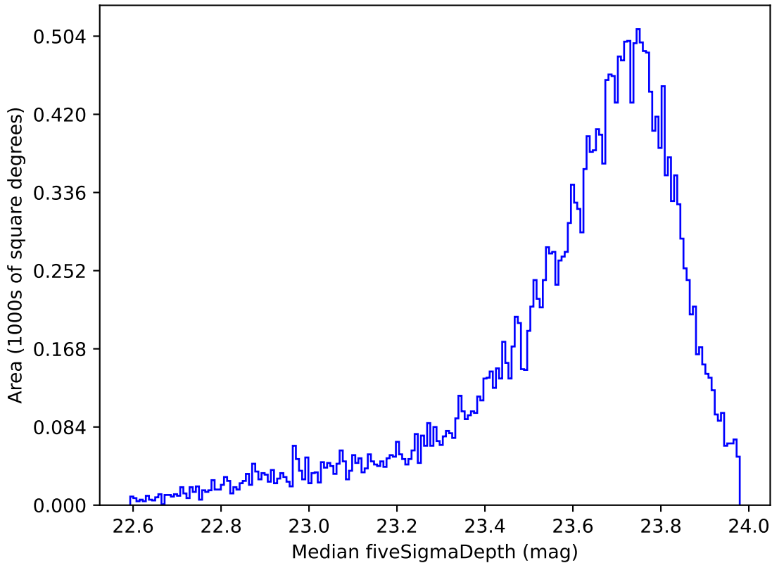
too_elab_r16_d2_griz_v3.4_10yrs Yr 1 i band: Median fiveSigmaDepth
