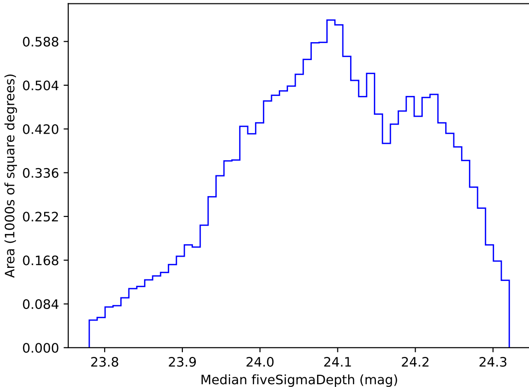
too_elab_r16_d2_griz_v3.4_10yrs WFD r band: Median fiveSigmaDepth
