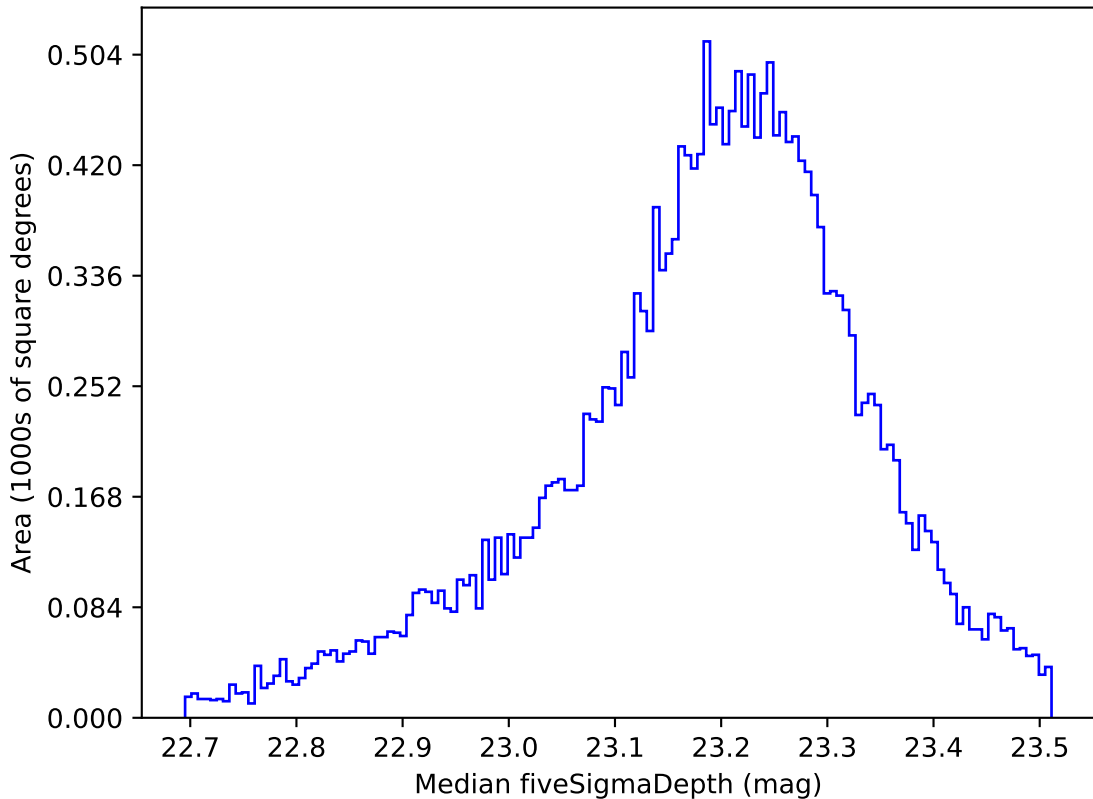
too_elab_r16_d2_griz_v3.4_10yrs All sky u band: Median fiveSigmaDepth
