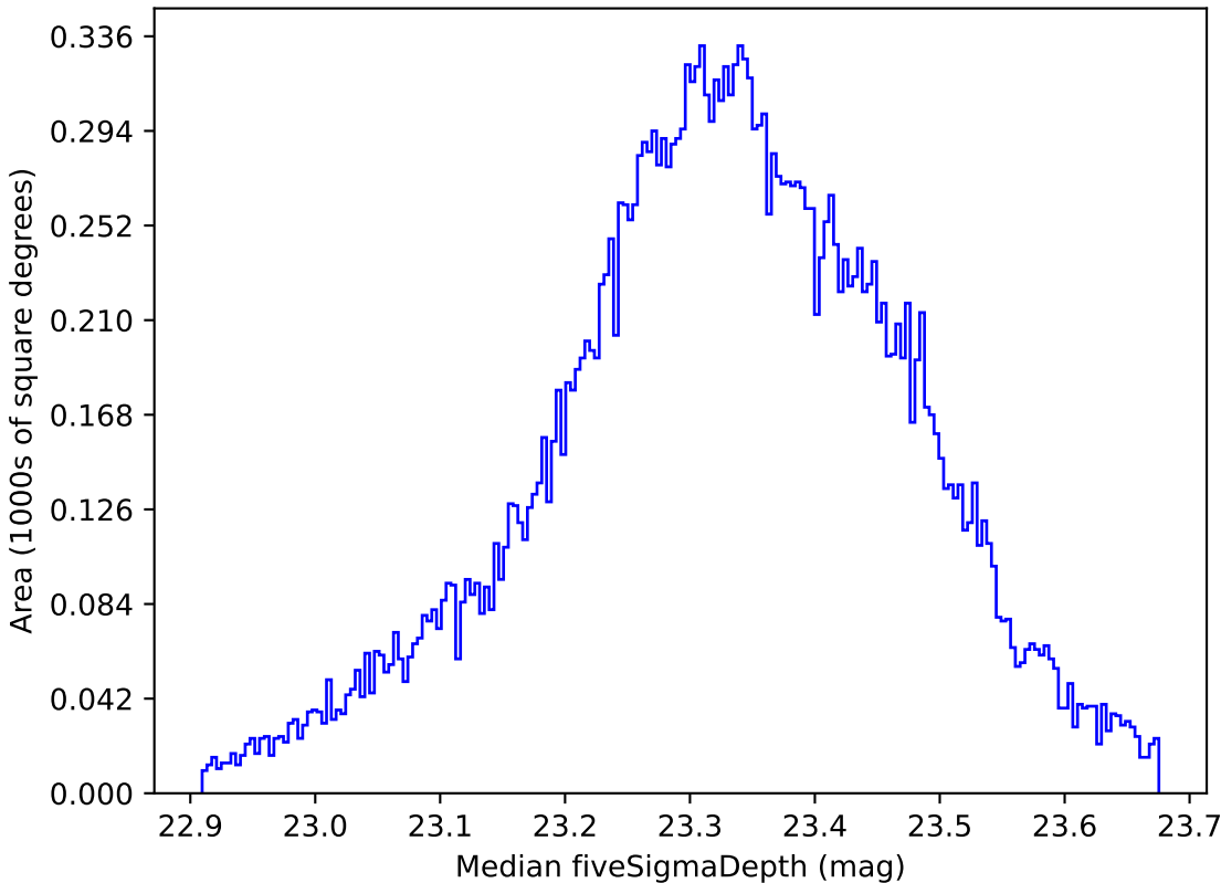
too_elab_r16_d2_griz_v3.4_10yrs All sky all bands: Median fiveSigmaDepth
